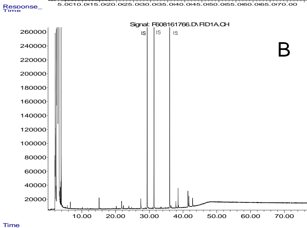
Figure 5: GC/FID chromatograms for the two water samples (A) FPN J17008-001 (Samson Pier) and (B) FPN J17008-002 (freshwater at end of other pier). #: n-alkane carbon number; Pr: pristane; Ph: phytane; UCM: unresolved complex mixture; IS: internal standards.
