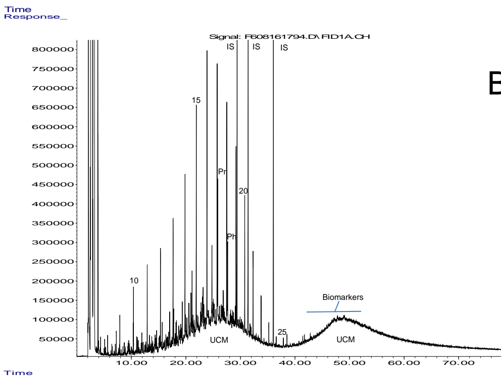
Figure 2: GC/FID chromatograms for the two source oil samples collected from the sunken Powhatan tugboat; (A) 2017-05-04-01-01 and (B) 2017-05-04-01-02. #: n-alkane carbon number; Pr: pristane; Ph: phytane; UCM: unresolved complex mixture; IS: internal standards.
