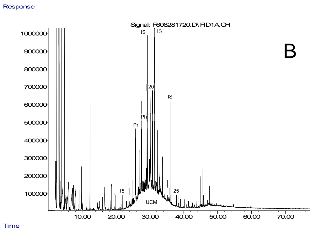
Figure 7: GC/FID chromatograms for the two sheen samples collected April 26, 2017; (A) FPN J17008-003 (boat ramp by jetty) and (B) FPN J17008-004 (Mosquito Trail). #: n-alkane carbon number; Pr: pristane; Ph: phytane; UCM: unresolved complex mixture; IS: internal standards.
